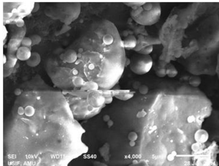
Fig. 1 SEM of the fly ash (10kV, x4000, 5µm)
