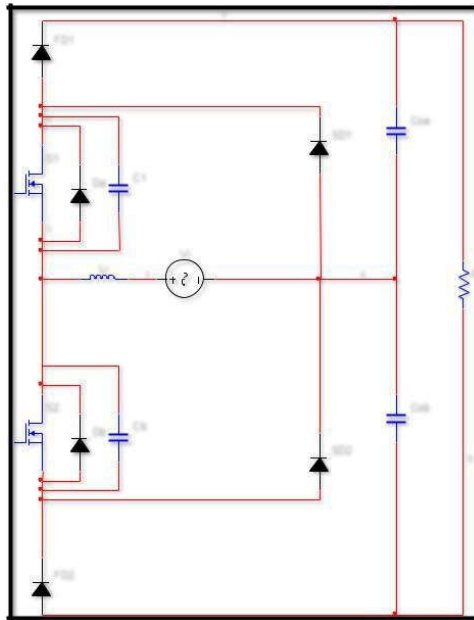
Figure 2: Proposed converter
