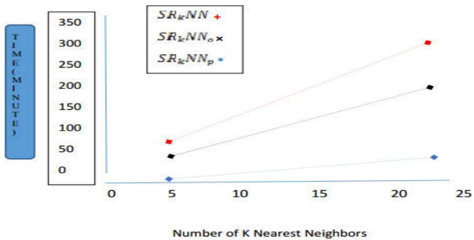
Efficiency gains of stage 1 for k= 1024
